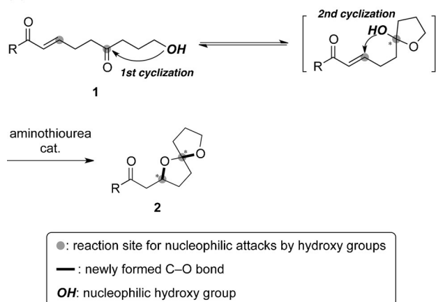
Scheme 1. Strategies for spiroketalization.
